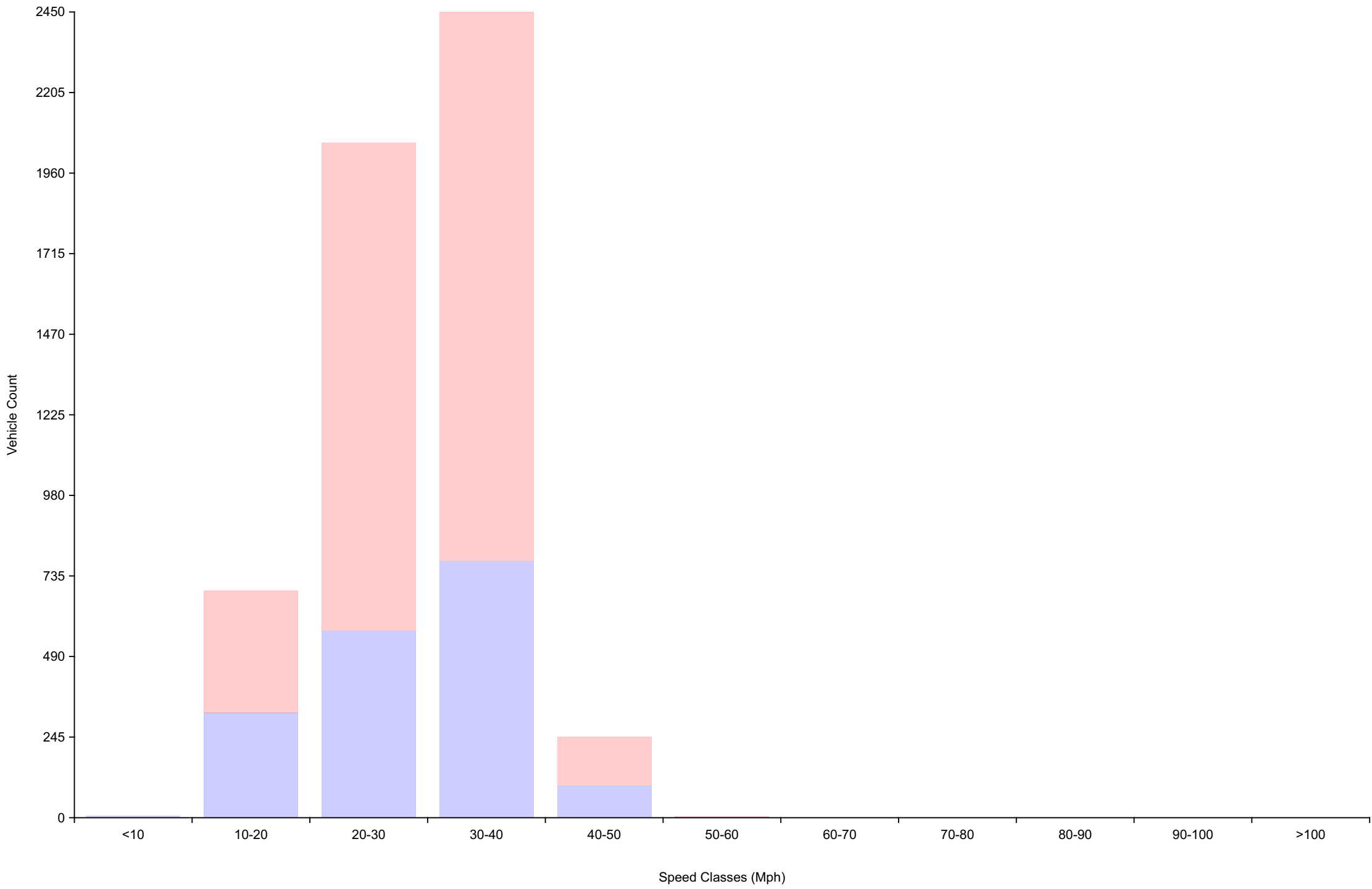
Vehicle Counts By Speed Class For week beginning Mon Mar 14 2022
